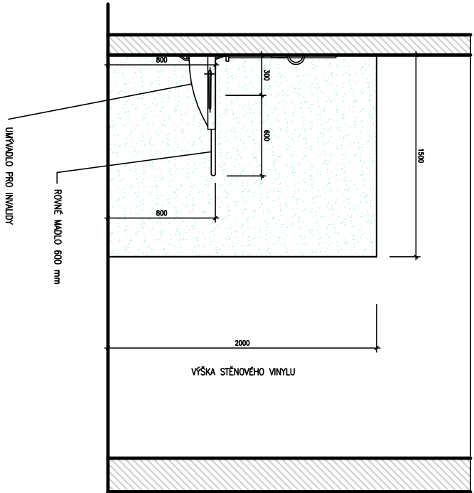
POHLED "C"
